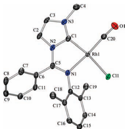
Figure 2. ORTEP drawing of 5 (hydrogens omitted for clarity, ellipsoids at 50% probability). Selected bond lengths (Å) and angles (deg): Rh–N(1), 2.131(2); Rh–Cl, 2.3665(6); Rh–C(1), 1.953(2); Rh–C(20), 1.813(3); C(5)–N(1), 1.293(3); C(5)–N(2), 1.386(3); C(1)–Rh–C(20), 97.39(11); C(20)–Rh–Cl, 90.38(8); Cl–Rh–N(1), 93.40(6); N(1)–Rh–C(1), 78.53(9).
